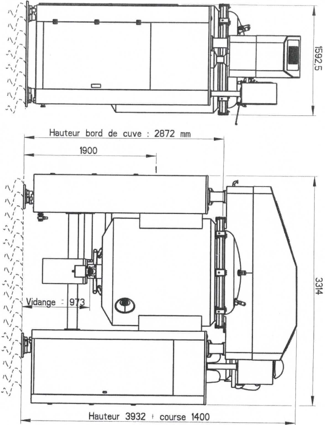
8.1.2 Dimensions B00165595-000
